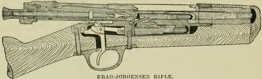
KRAJ-JORGENSEN RIFLE.
